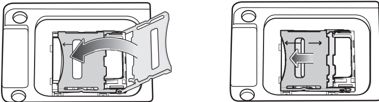
Figure 12 Lock microSD Card Holder
