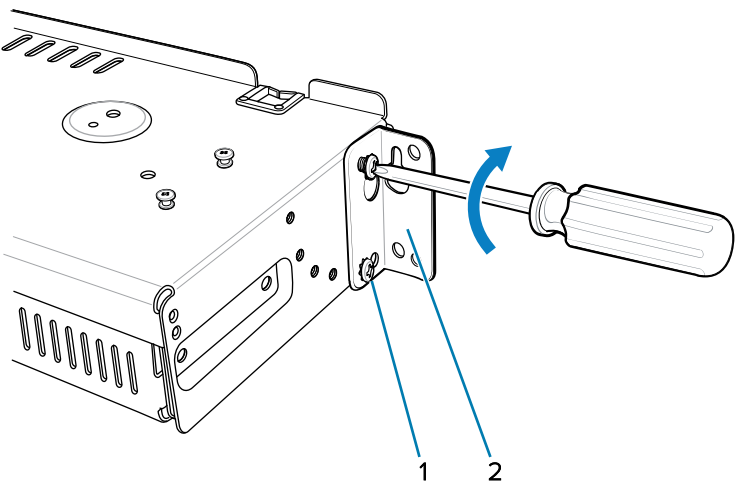
Figure 51 Flange Horizontal Position (5-Slot Cradles)
