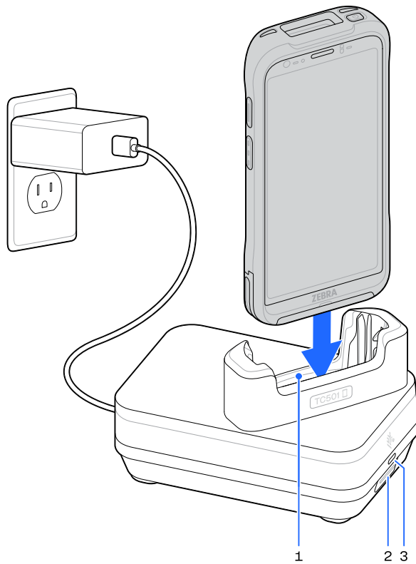
Figure 35 1-Slot Ethernet Rugged Charging Cradle
