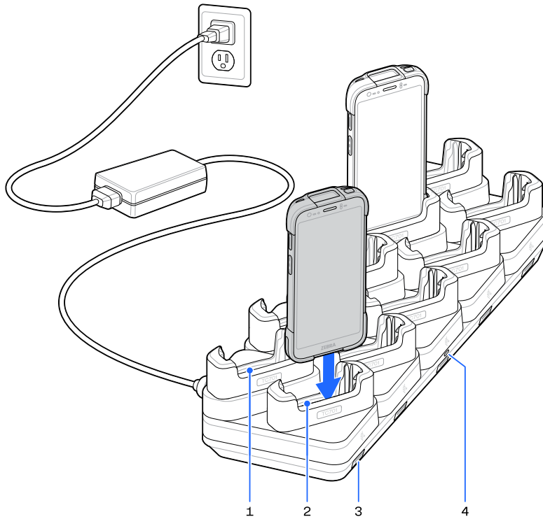
Figure 41 5-Slot 10-Devices Charging Cradle
