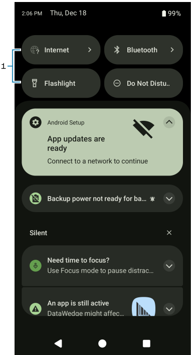
Figure 6 Notification Panel
