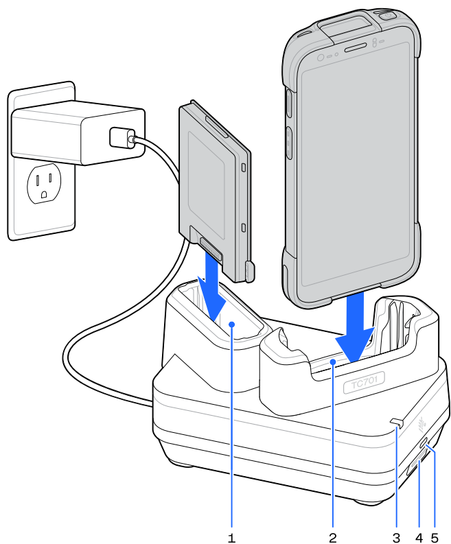
Figure 36 1-Slot Device and Spare Battery Ethernet Charging Cradle
