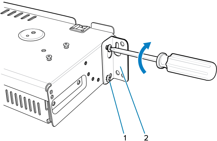
Figure 42 Flange Horizontal Position (5-Slot Cradles)
