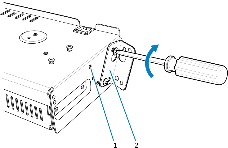
Figure 43 Flange 25° Position (4-Slot Battery Chargers)
