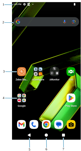
Figure 4 Home Screen
