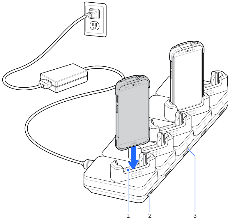
Figure 38 5-Slot Fast-Charging Cradle
