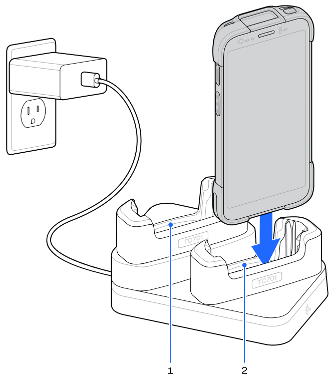
Figure 34 1-Slot 2-Device Charging Cradle
