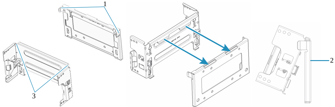
Figure 44 MT4200 Quick Release Mount Assembly
