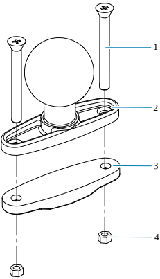
Figure 41 MT3507 Optional Mount Kits
