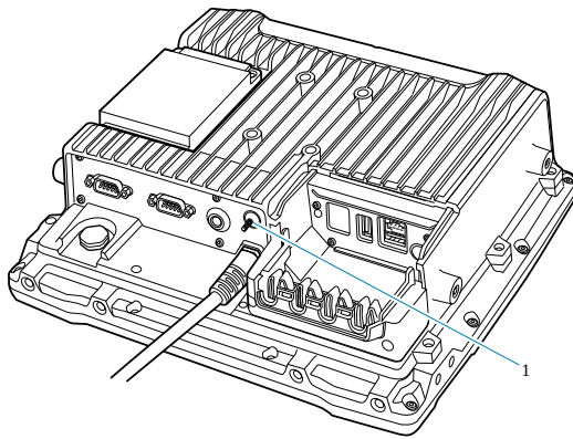
Figure 6 Ground Lug
