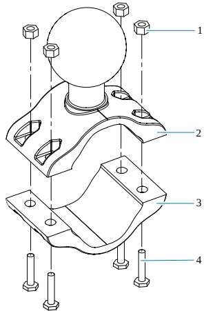
Figure 43 MT3510 Optional Mount Kit
