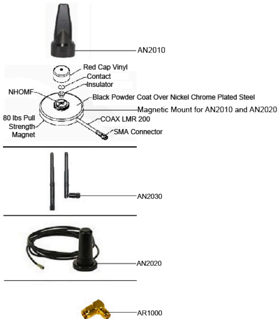
Figure 38 VC8300 Antenna Options
