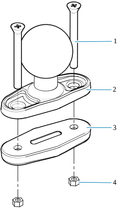
Figure 40 MT3505 Optional Mount Kits
