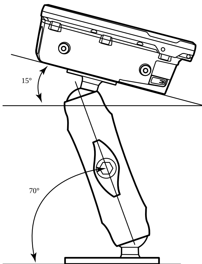
Figure 39 Orientation of Vehicle-Mount Assembly
