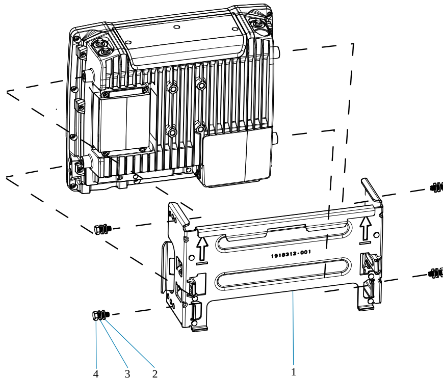
Figure 45 VC8300 and MT4200 Assembly
