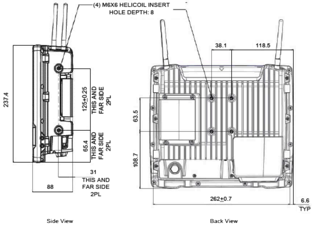
Figure 46 Drill Hole Dimensions
