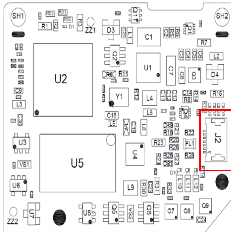
Figure 4 - Top View
