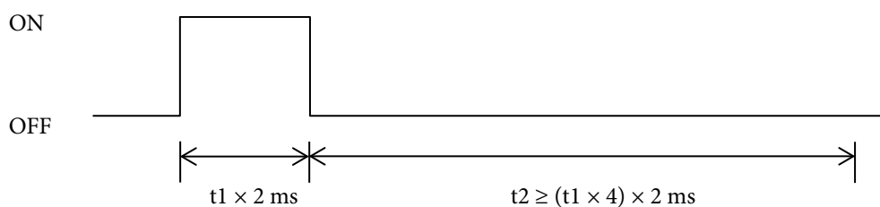
Figure C.1.1 Drawer Drive Signal Waveform
