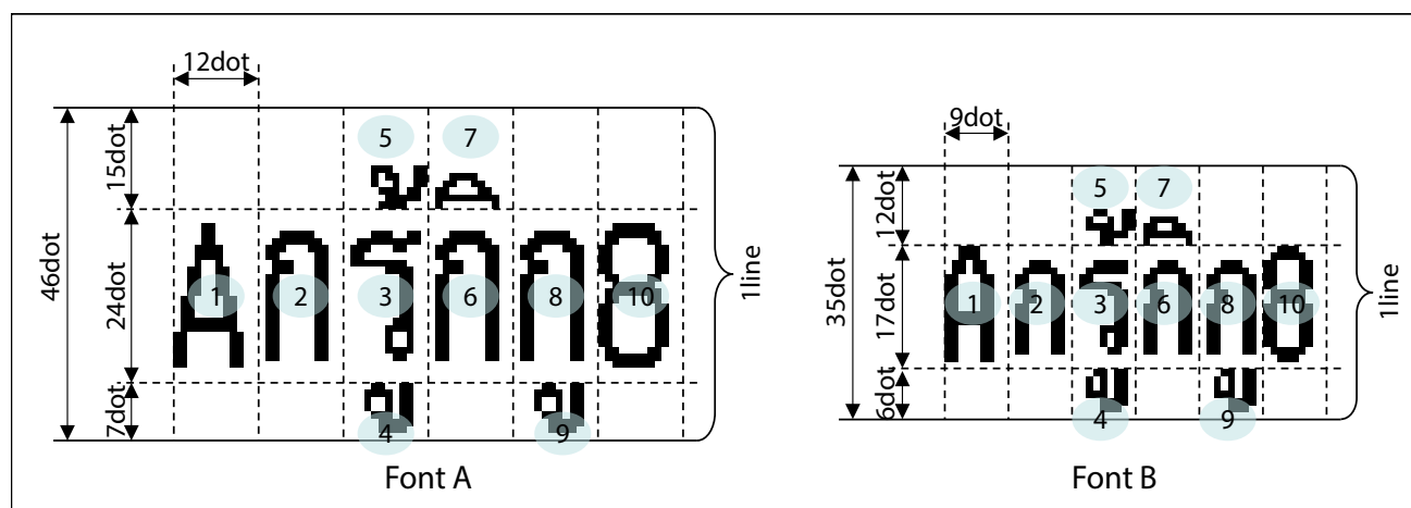
Figure K.2.1 Thai Character 1-pass Print Mode Fonts A and B
