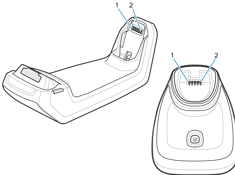
Figure 6 Cradle Pin-Outs
