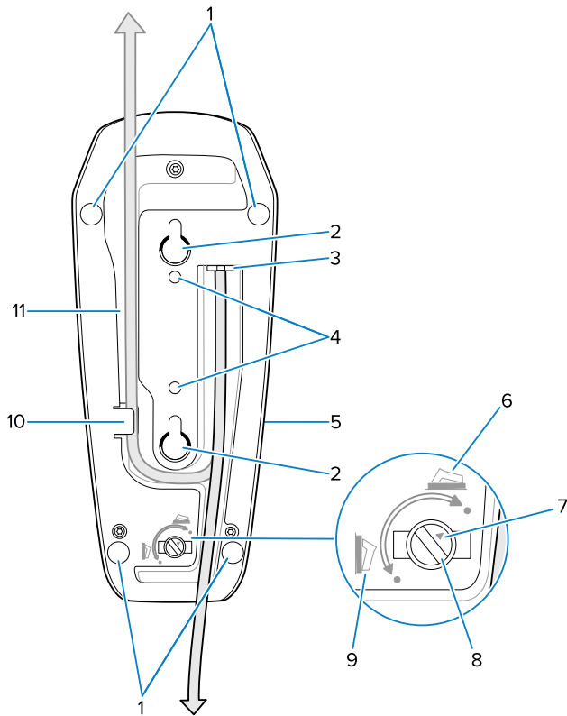
Figure 3 Bottom View
