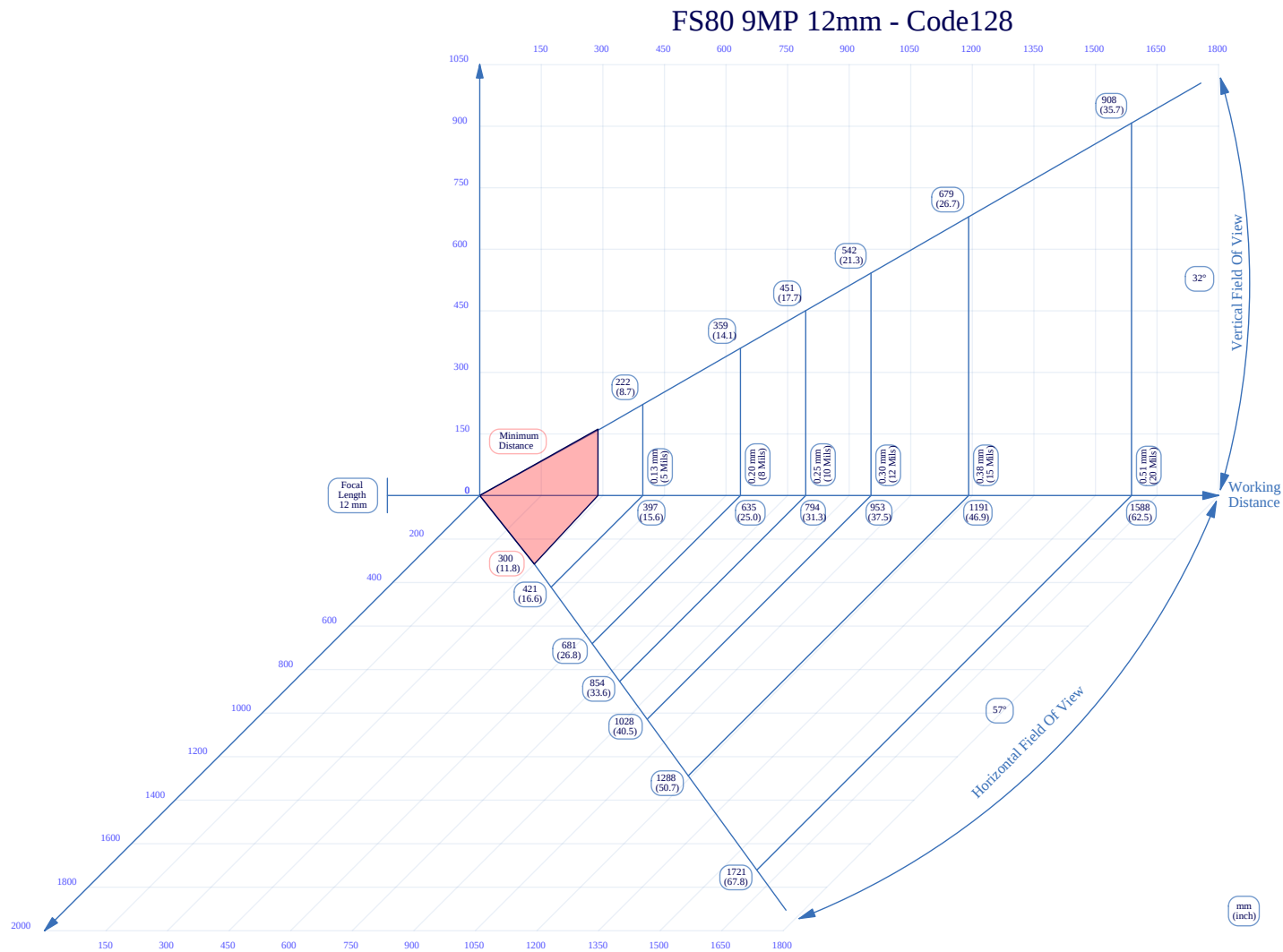
Figure 43 12mm C-Mount Lens Reading Code128
