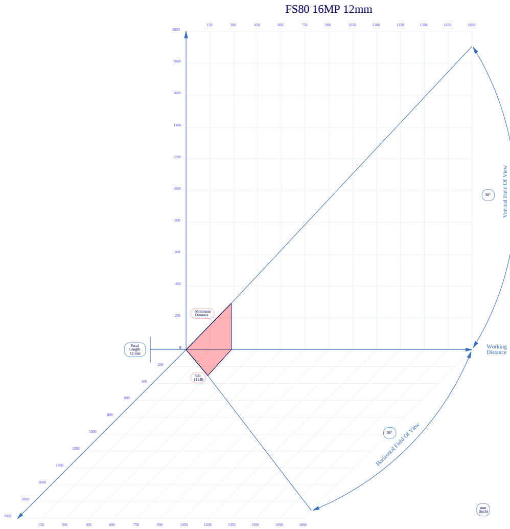
Figure 72 12mm C-Mount Lens Reading Distance
