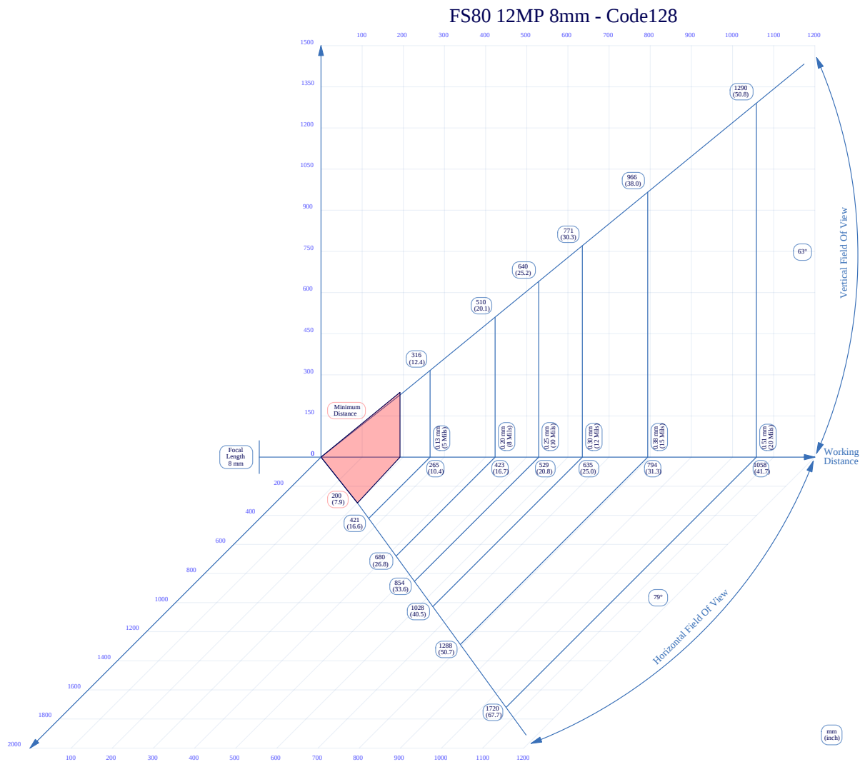
Figure 55 8mm C-Mount Lens Reading Code128
