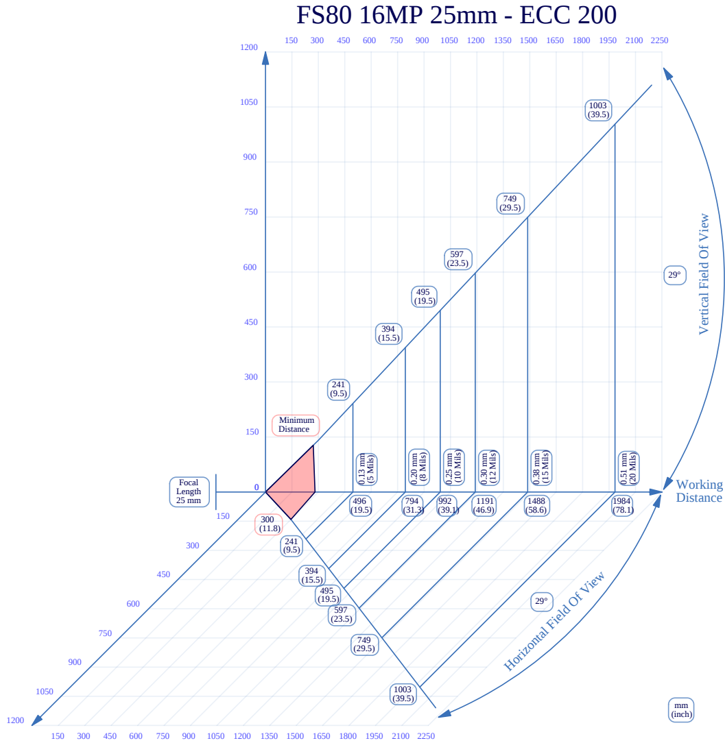
Figure 80 25mm C-Mount Lens Reading ECC 200
