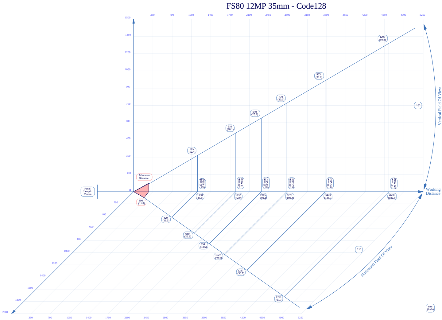
Figure 67 35mm C-Mount Lens Reading Code128
