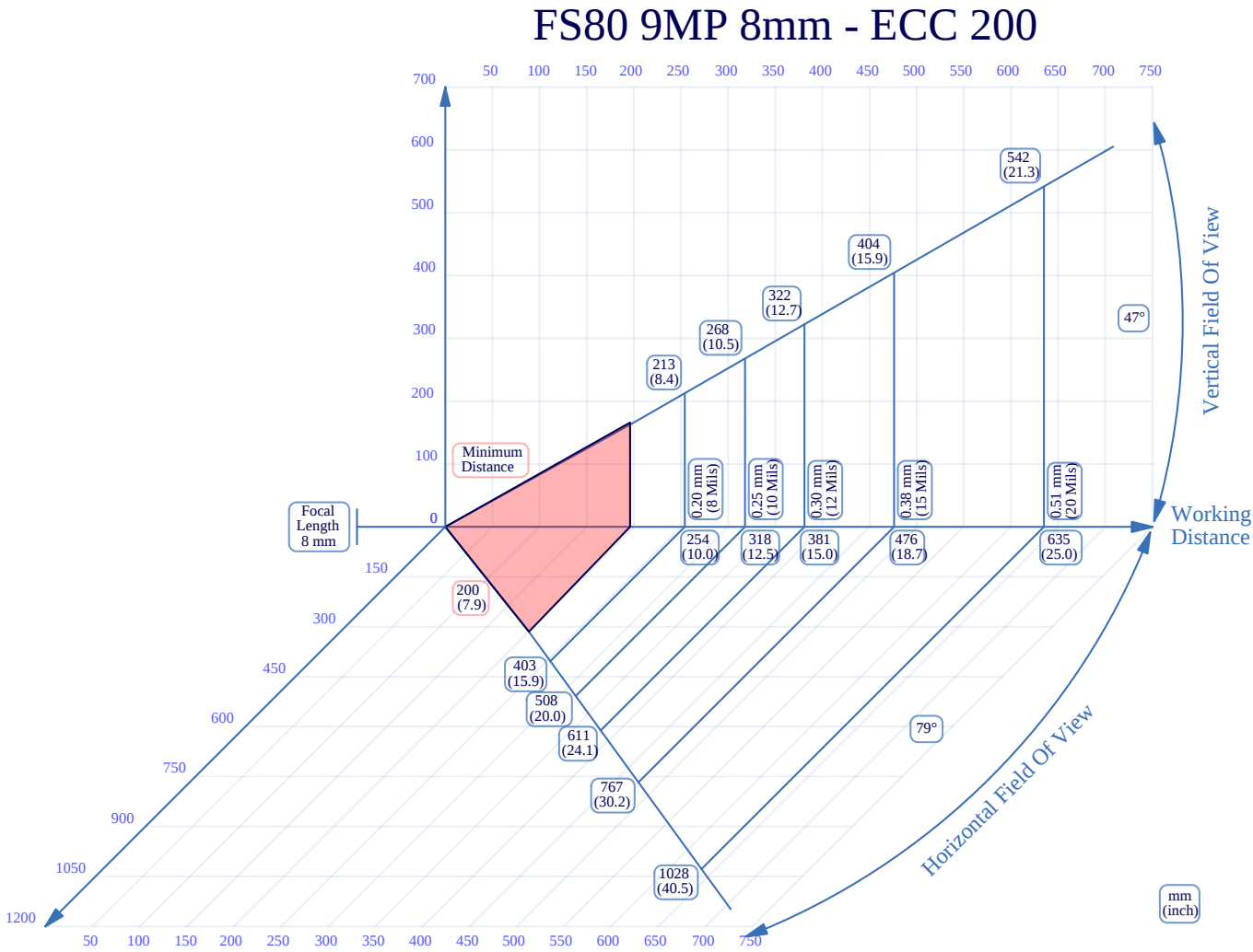
Figure 41 8mm C-Mount Lens Reading ECC 200
