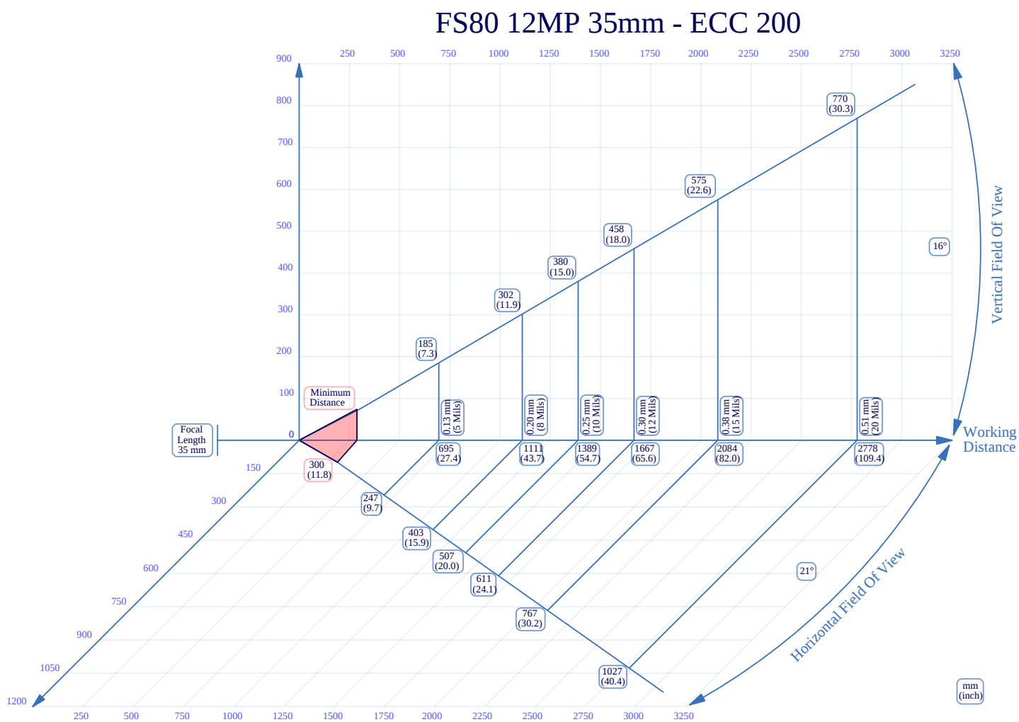
Figure 68 35mm C-Mount Lens Reading ECC 200
