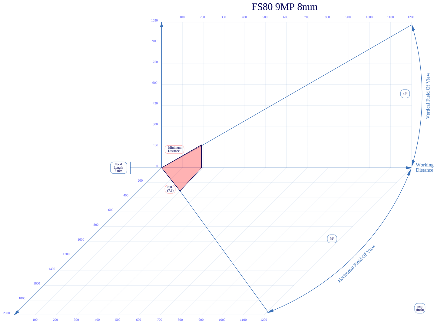
Figure 39 8mm C-Mount Lens Reading Distance
