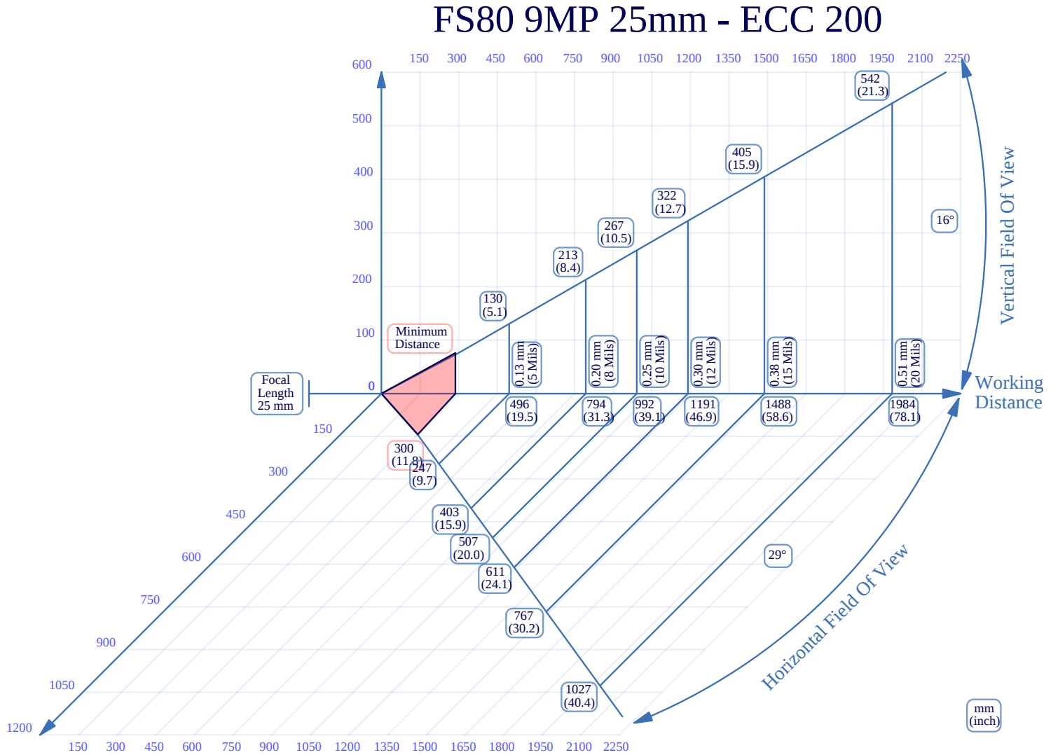
Figure 50 25mm C-Mount Lens Reading ECC 200
