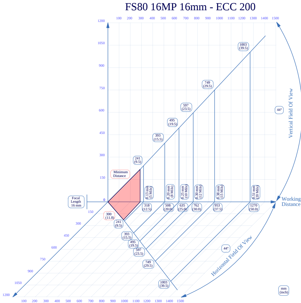
Figure 77 16mm C-Mount Lens Reading ECC 200
