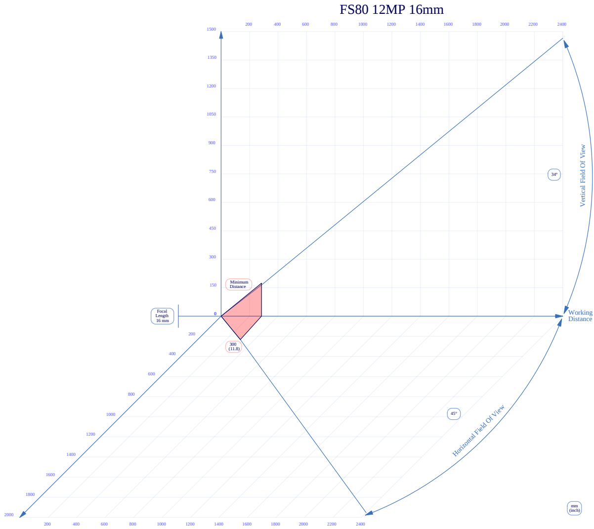
Figure 60 16mm C-Mount Lens Reading Distance
