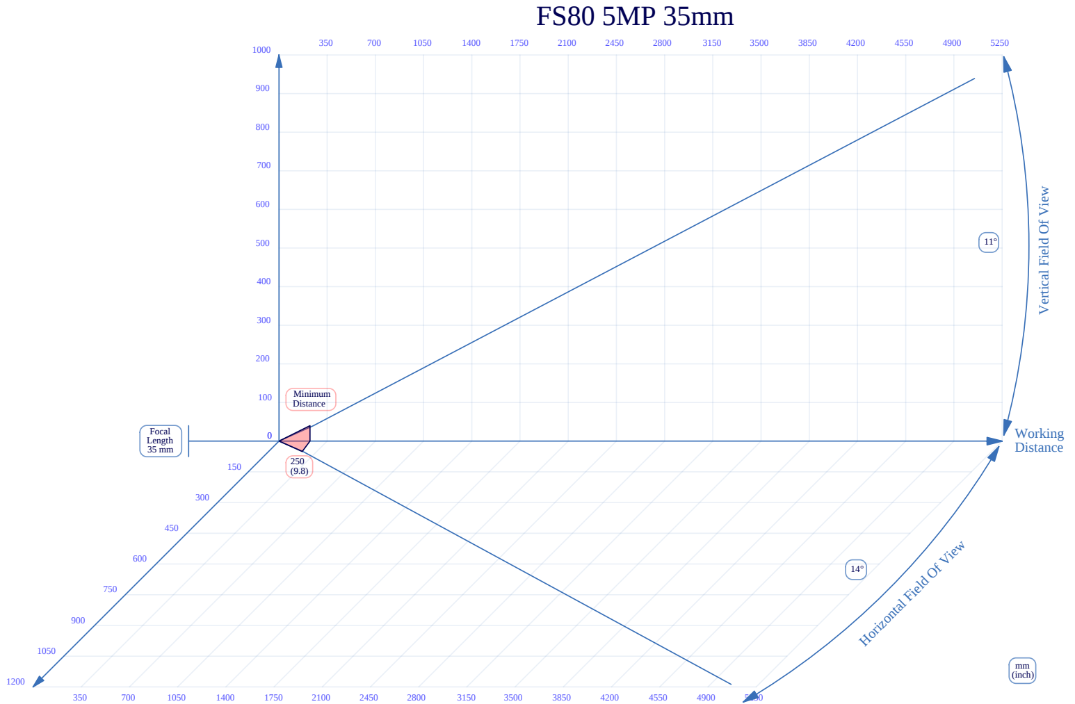
Figure 36 35mm C-Mount Lens Reading Distance
