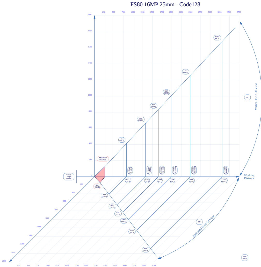
Figure 79 25mm C-Mount Lens Reading Code128
