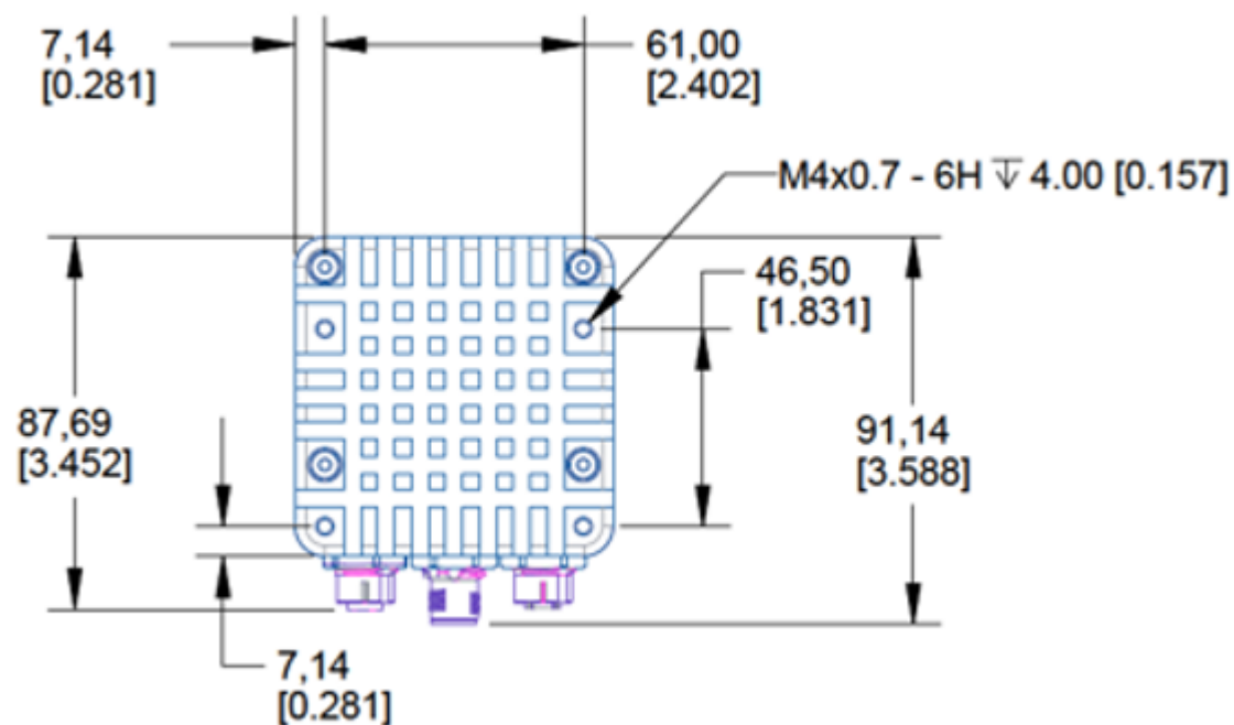
Figure 21 FS80 Dimensional Drawing - Side View
