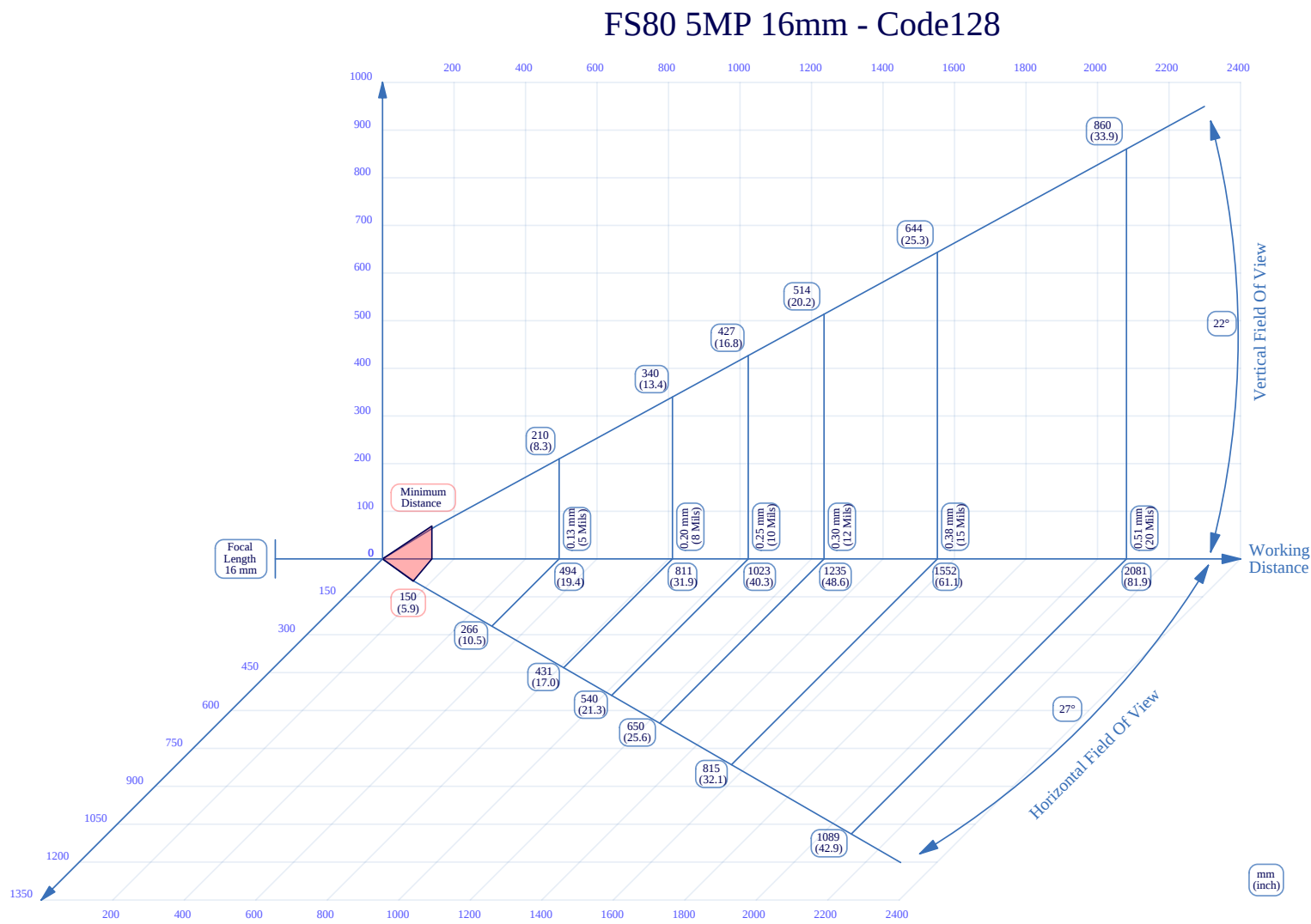
Figure 31 16mm C-Mount Lens Reading Code128
