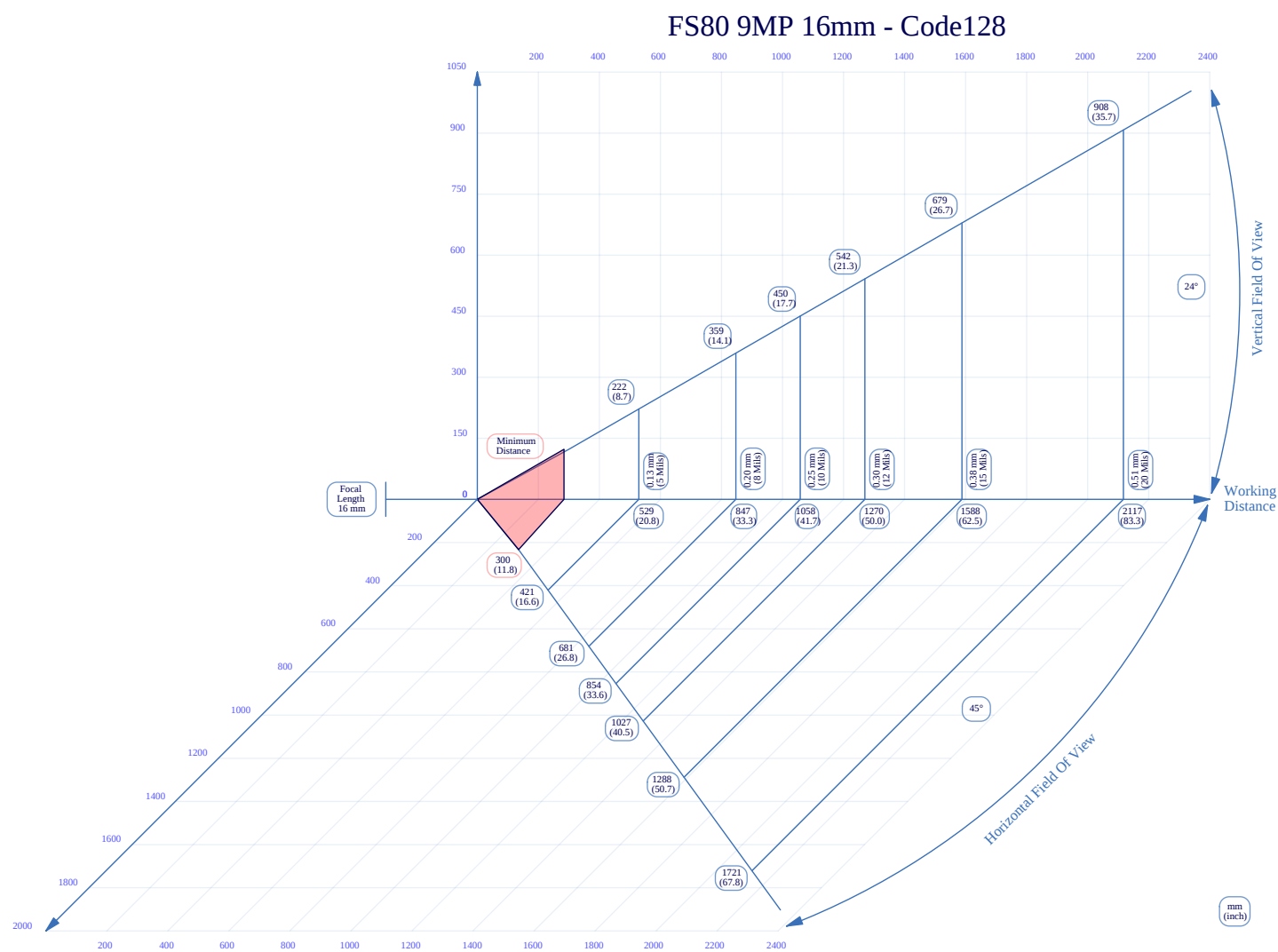
Figure 46 16mm C-Mount Lens Reading Code128
