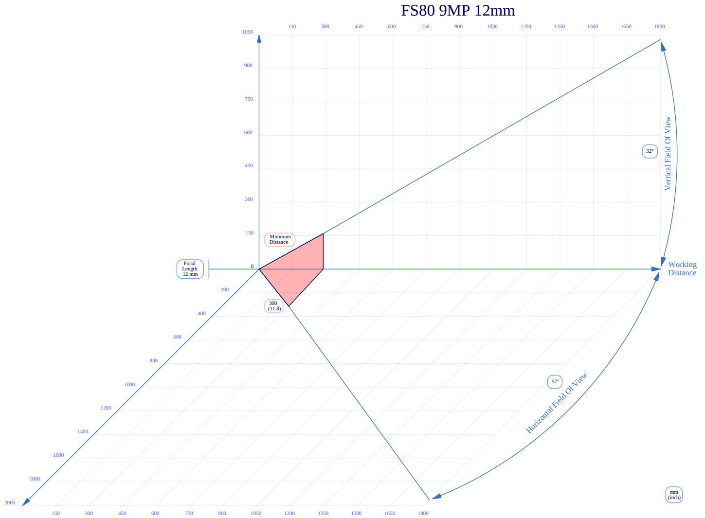
Figure 42 12mm C-Mount Lens Reading Distance
