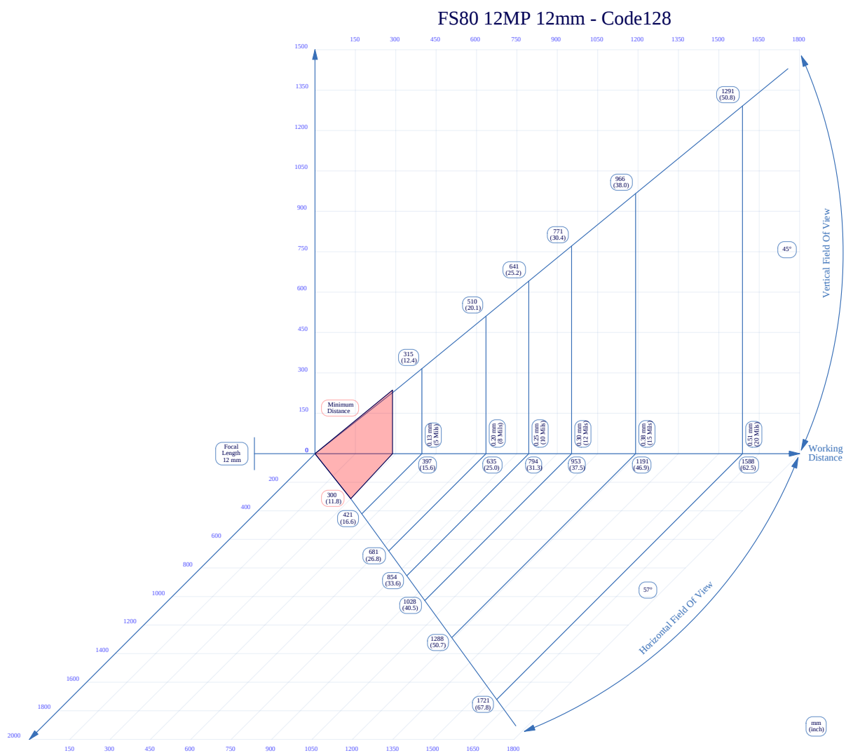
Figure 58 12mm C-Mount Lens Reading Code128
