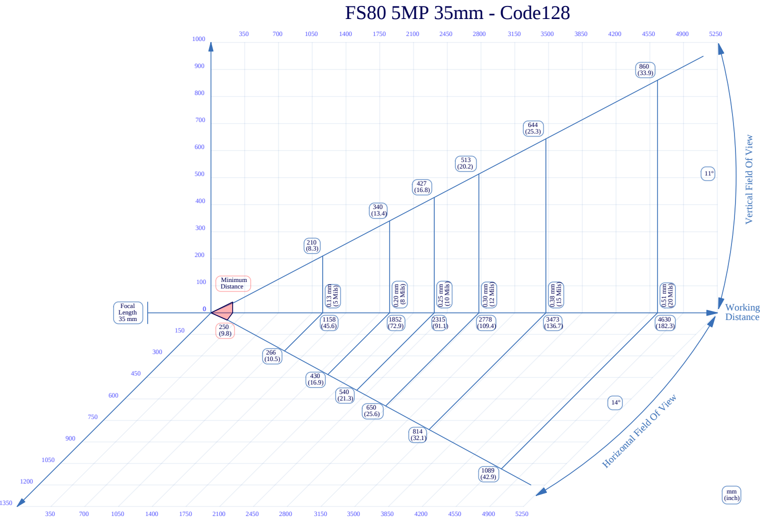
Figure 37 35mm C-Mount Lens Reading Code128
