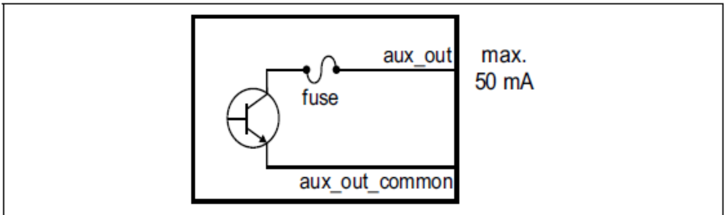
Figure 5 On-Board Fuse
