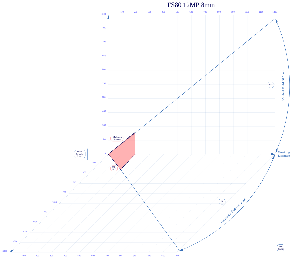
Figure 54 8mm C-Mount Lens Reading Distance
