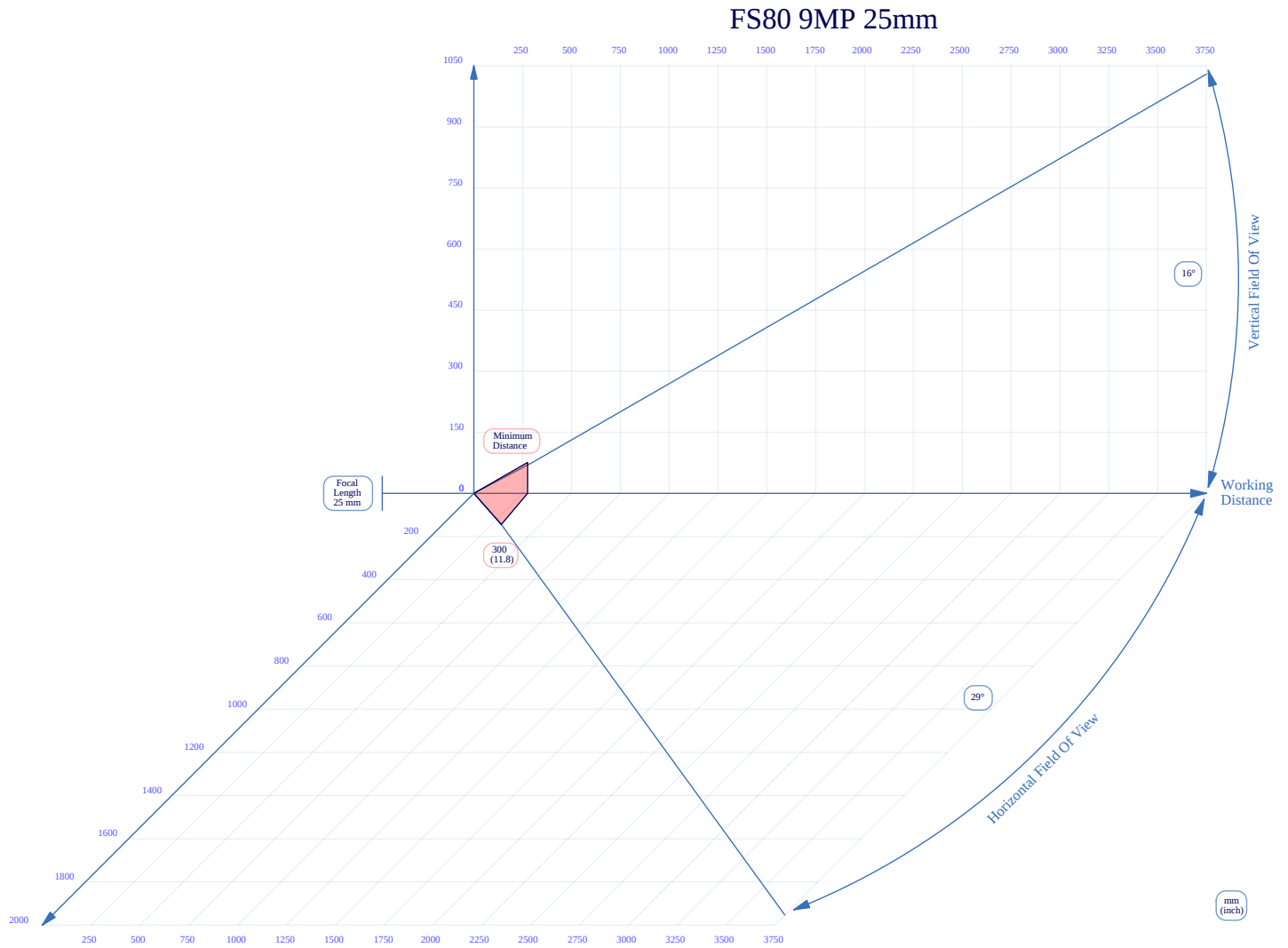
Figure 48 25mm C-Mount Lens Reading Distance
