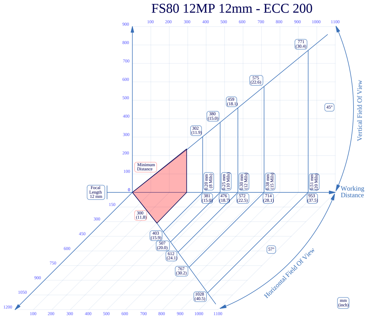
Figure 59 12mm C-Mount Lens Reading ECC 200
