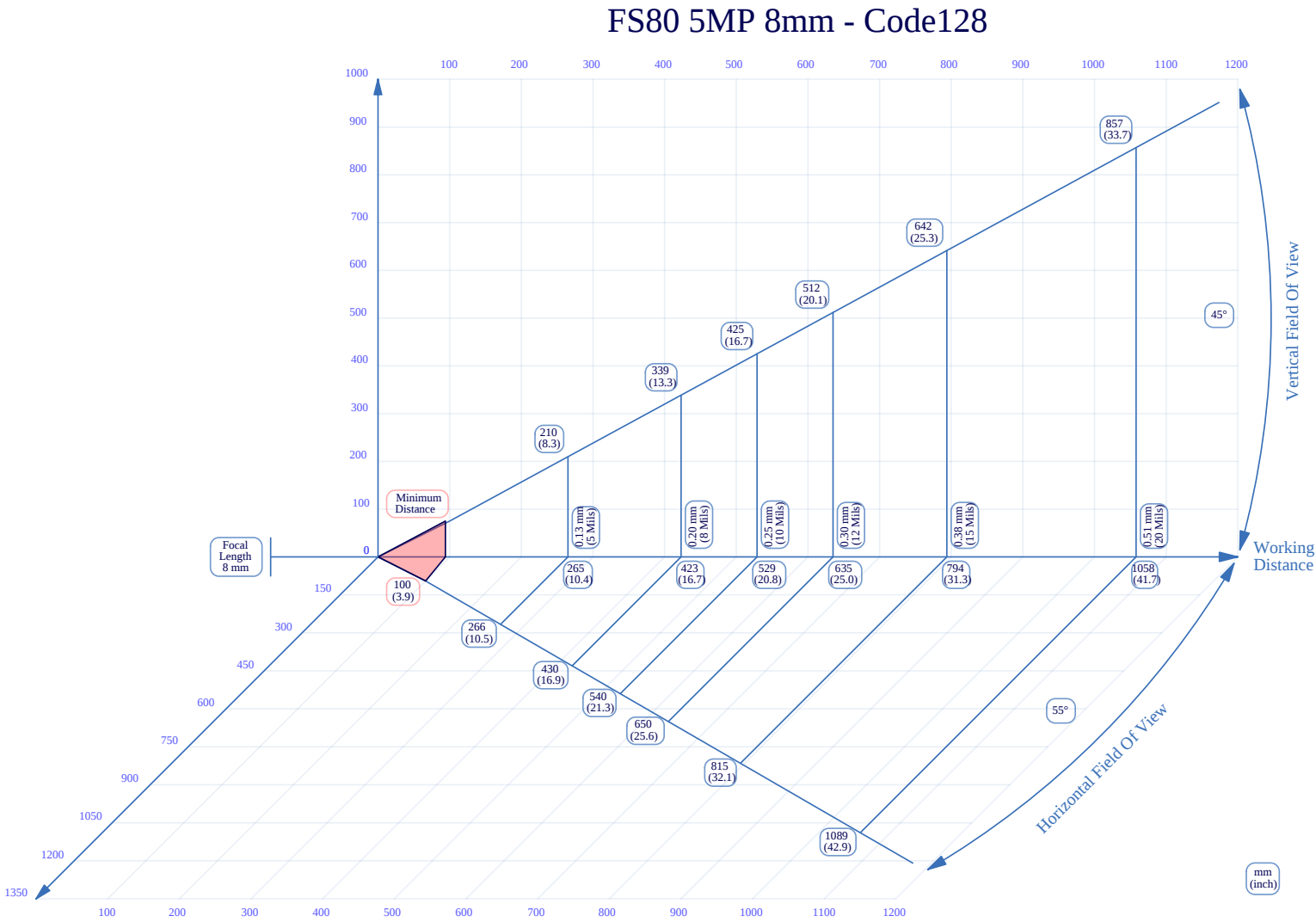
Figure 25 8mm C-Mount Lens Reading Code128
