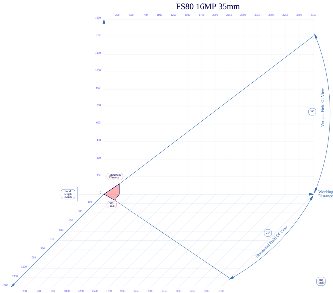
Figure 81 35mm C-Mount Lens Reading Distance
