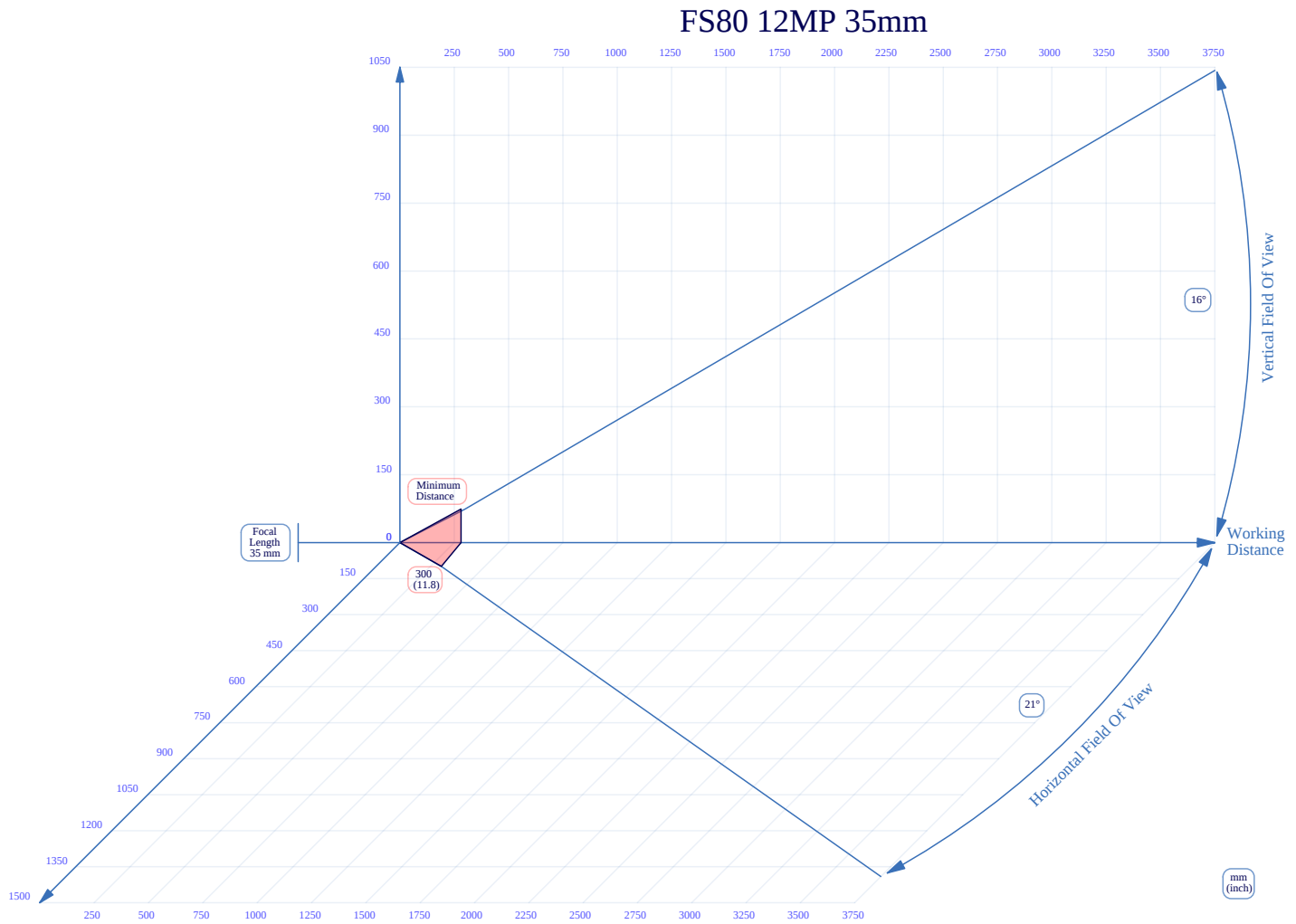
Figure 66 35mm C-Mount Lens Reading Distance
