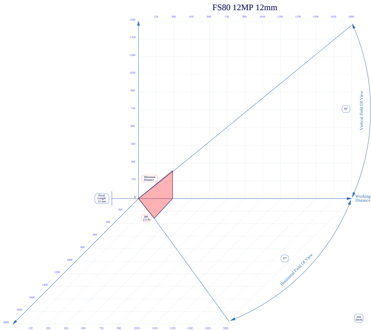
Figure 57 12mm C-Mount Lens Reading Distance
