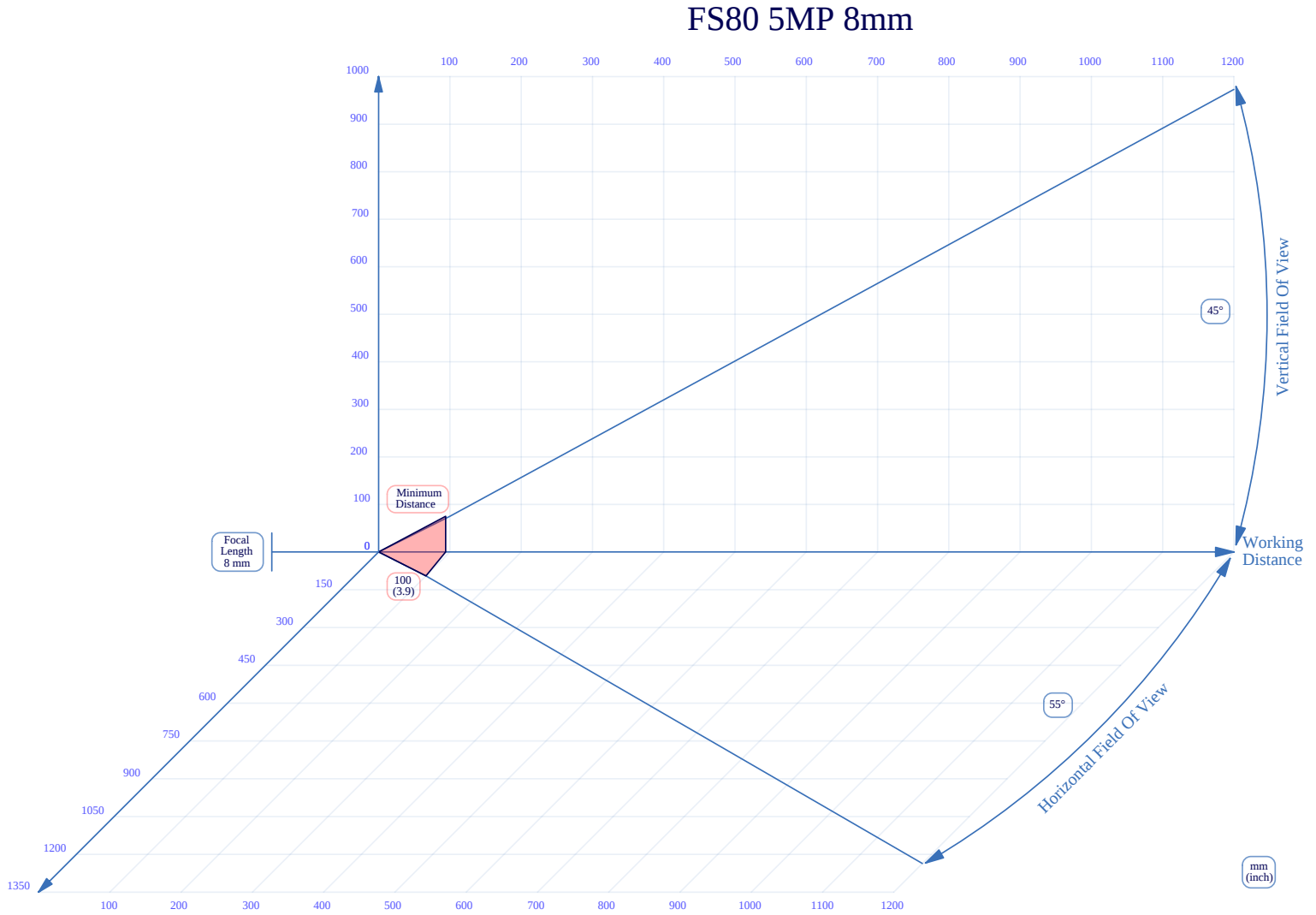
Figure 24 8mm C-Mount Lens Reading Distance
