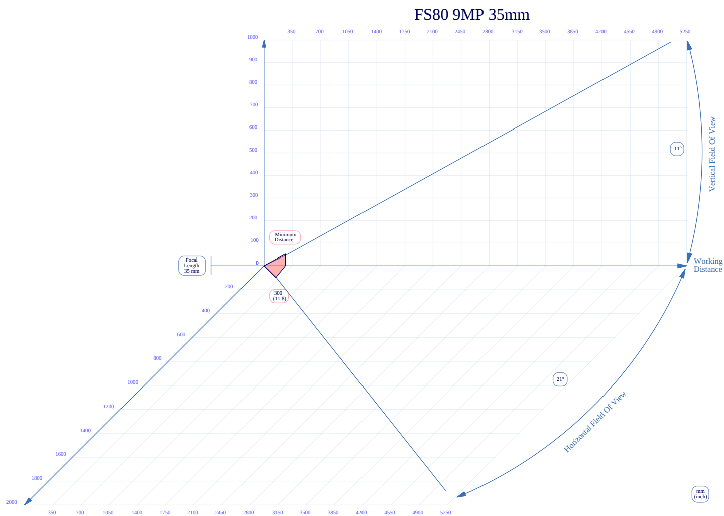
Figure 51 35mm C-Mount Lens Reading Distance
