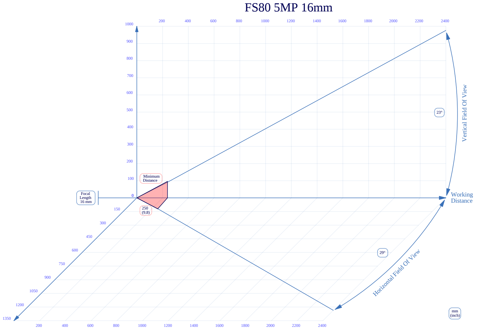
Figure 30 16mm C-Mount Lens Reading Distance
