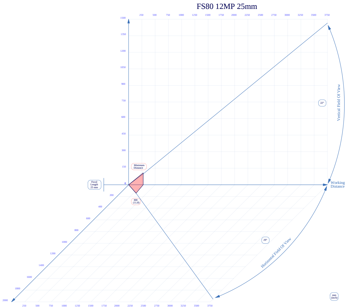
Figure 63 25mm C-Mount Lens Reading Distance
