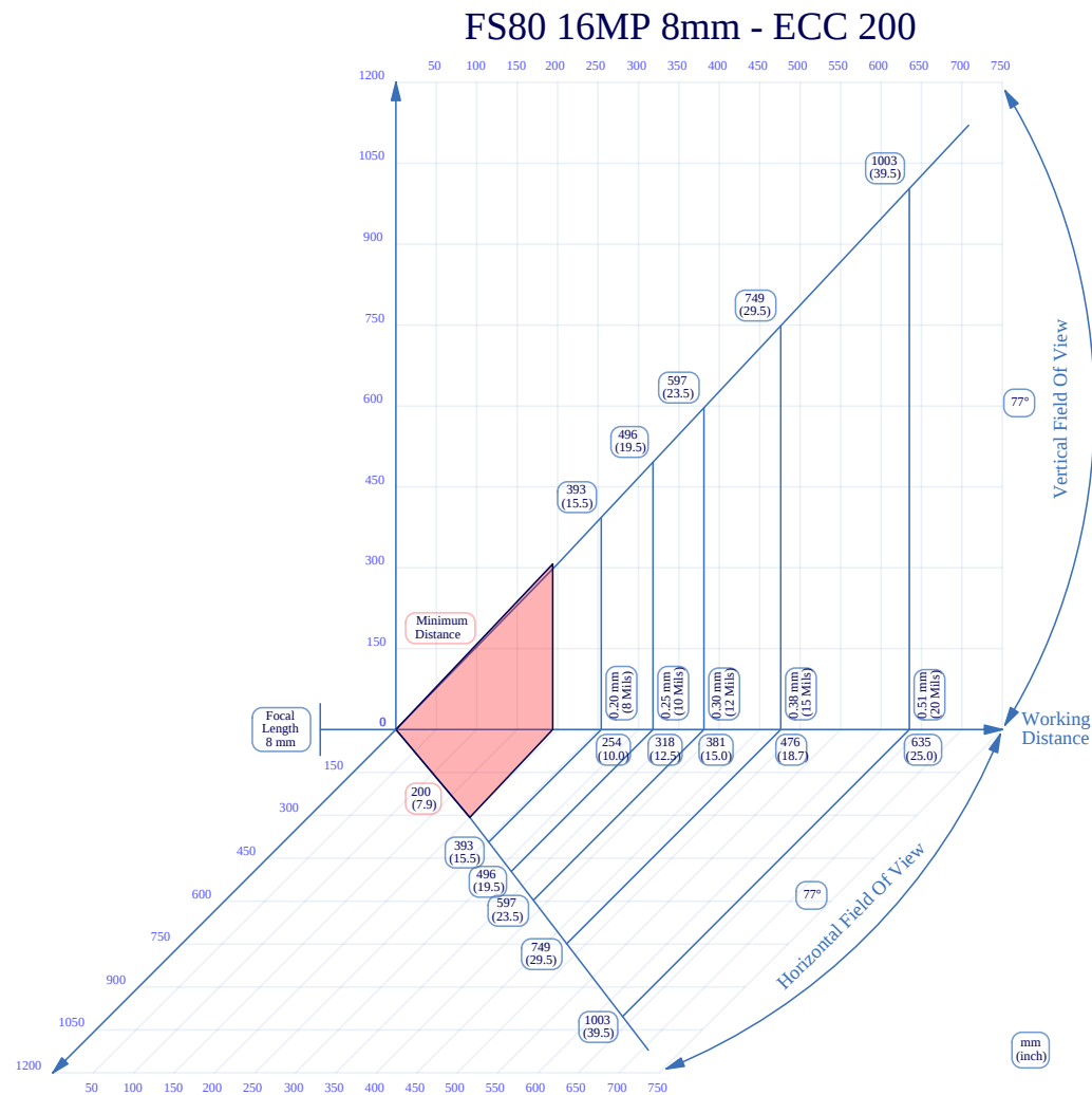
Figure 71 8mm C-Mount Lens Reading ECC 200
