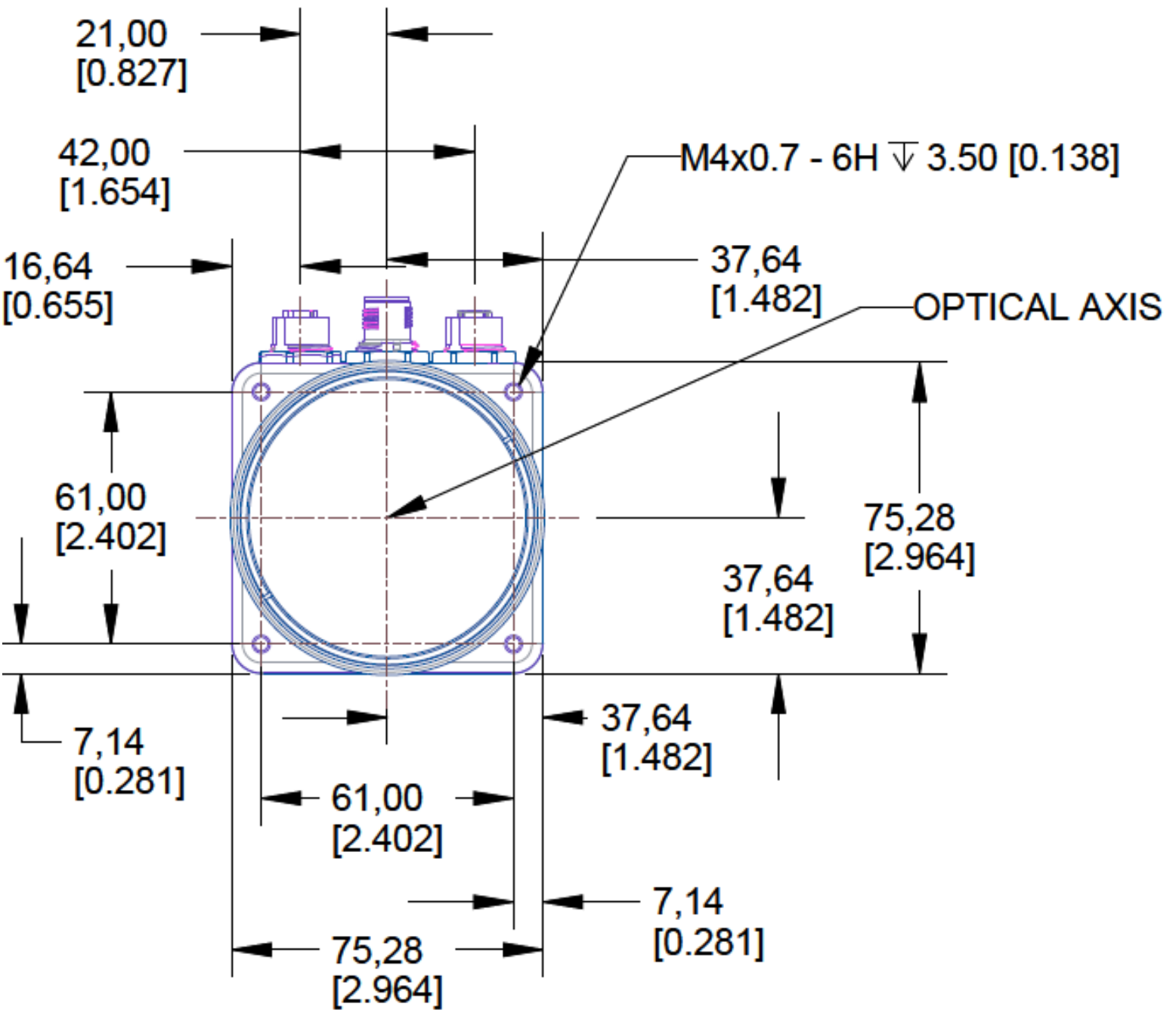
Figure 22 FS80 and Lens Cover Dimensional Drawing - Top View
