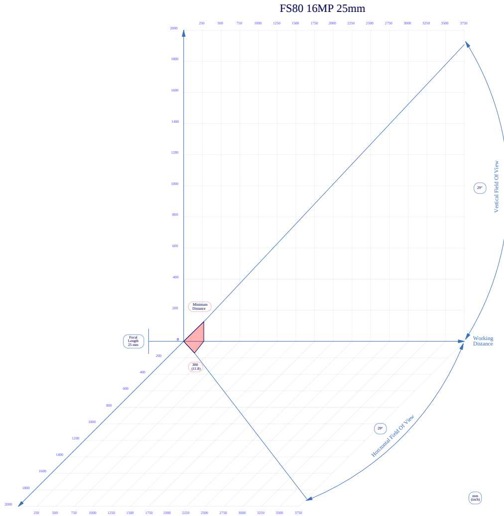
Figure 78 25mm C-Mount Lens Reading Distance
