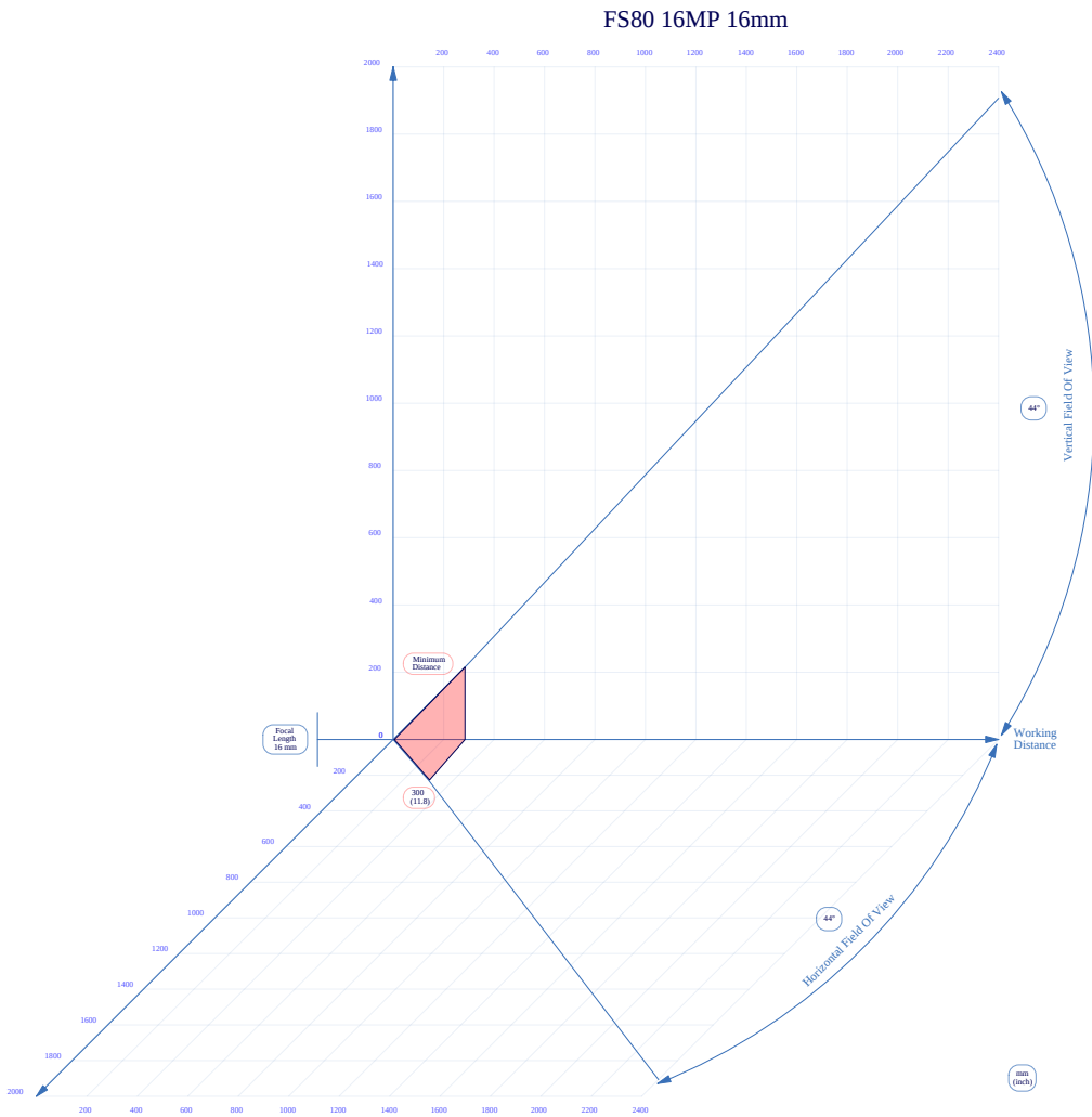
Figure 75 16mm C-Mount Lens Reading Distance
