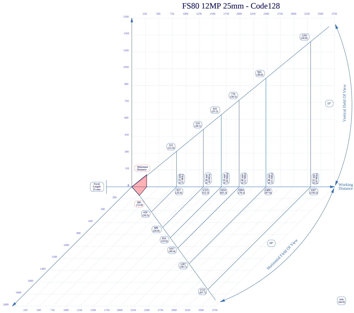
Figure 64 25mm C-Mount Lens Reading Code128
