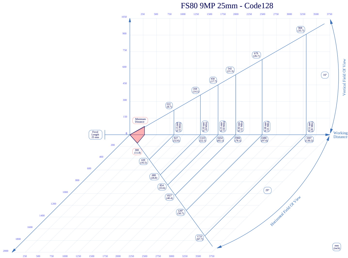
Figure 49 25mm C-Mount Lens Reading Code128
