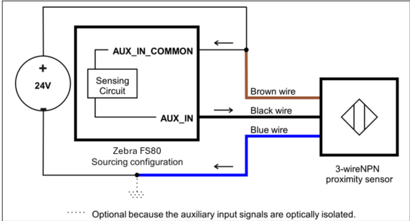
Figure 15 3-Wire NPN Proximity Sensor
