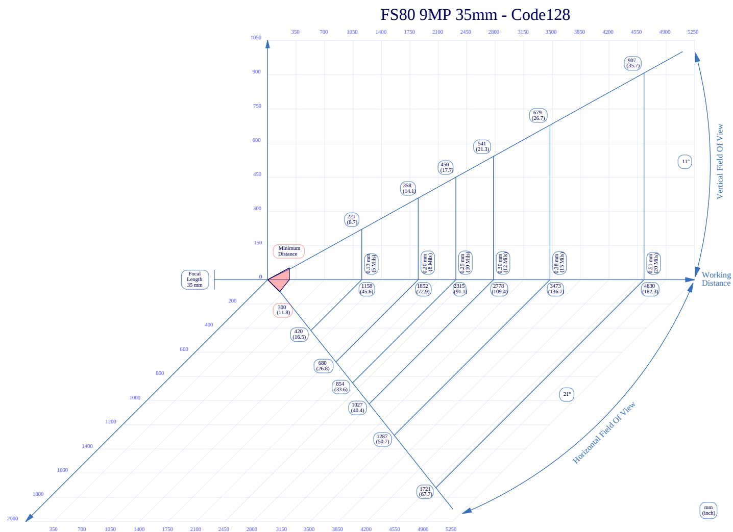
Figure 52 35mm C-Mount Lens Reading Code128
