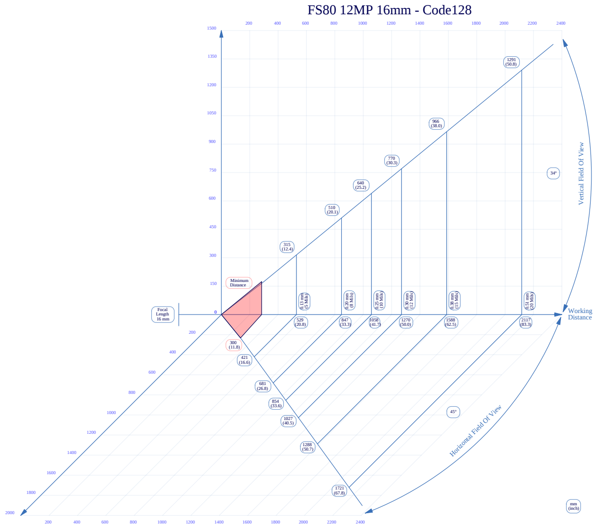
Figure 61 16mm C-Mount Lens Reading Code128
