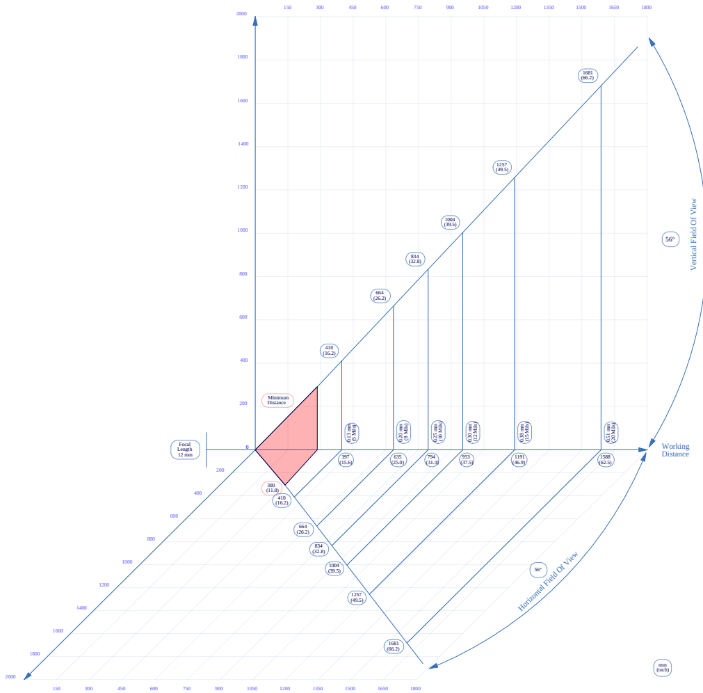
FS80 16MP 12mm - Code128
