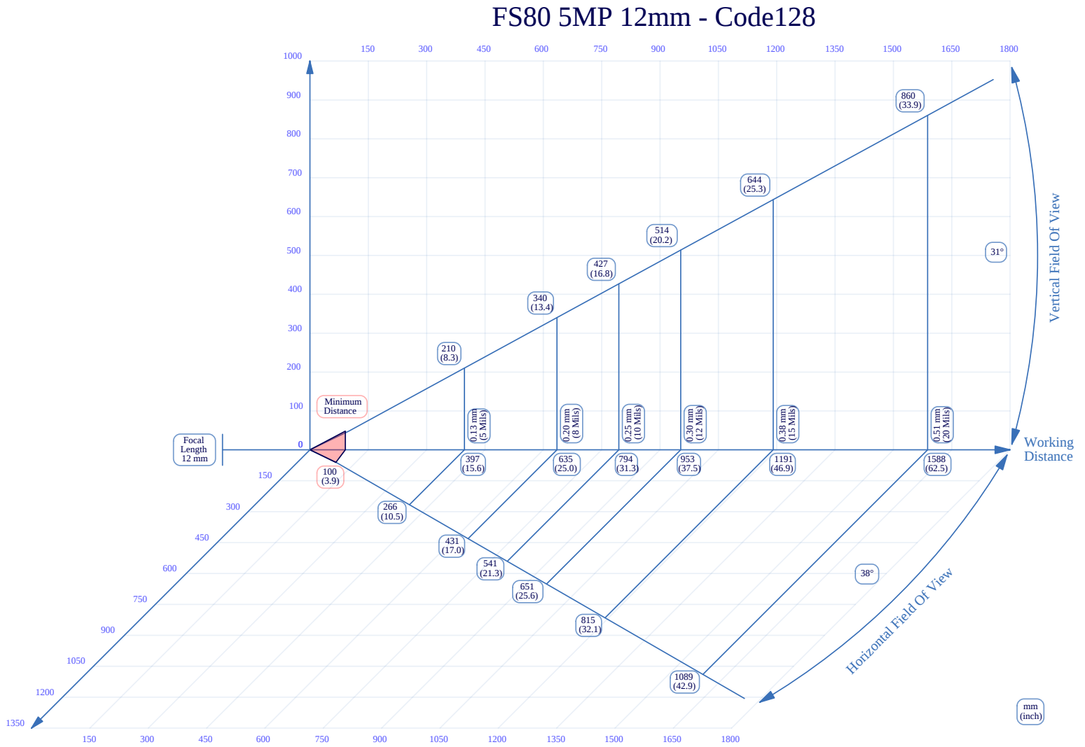
Figure 28 12mm C-Mount Lens Reading Code128
