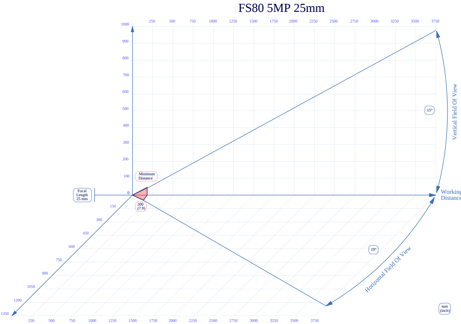
Figure 33 25mm C-Mount Lens Reading Distance
