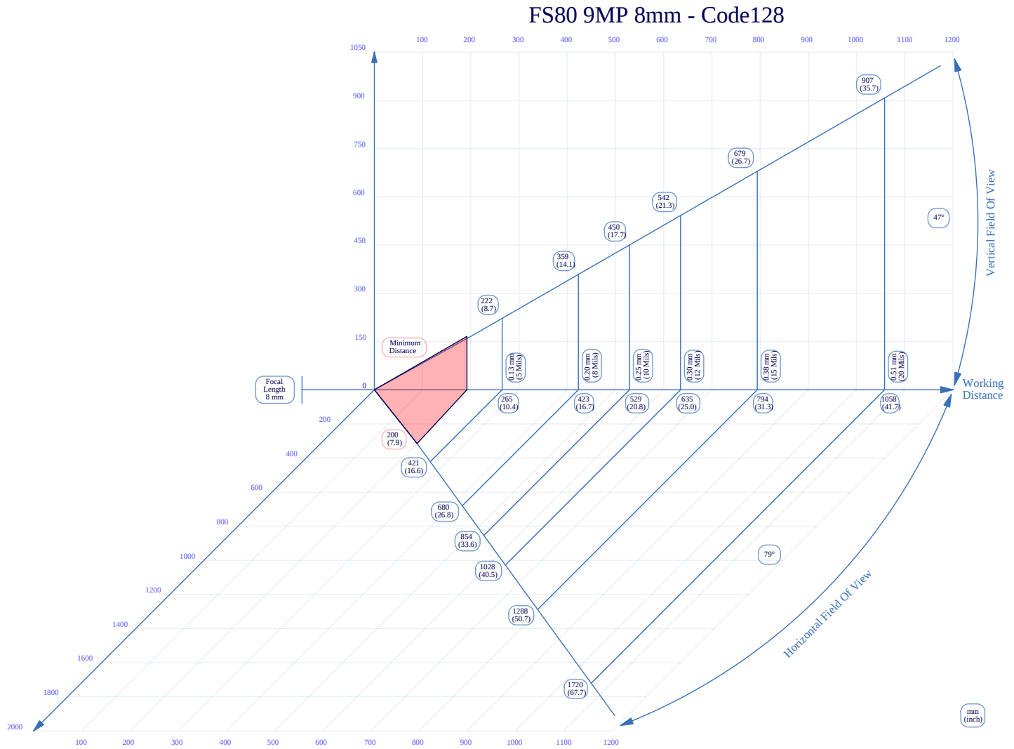
Figure 40 8mm C-Mount Lens Reading Code128
