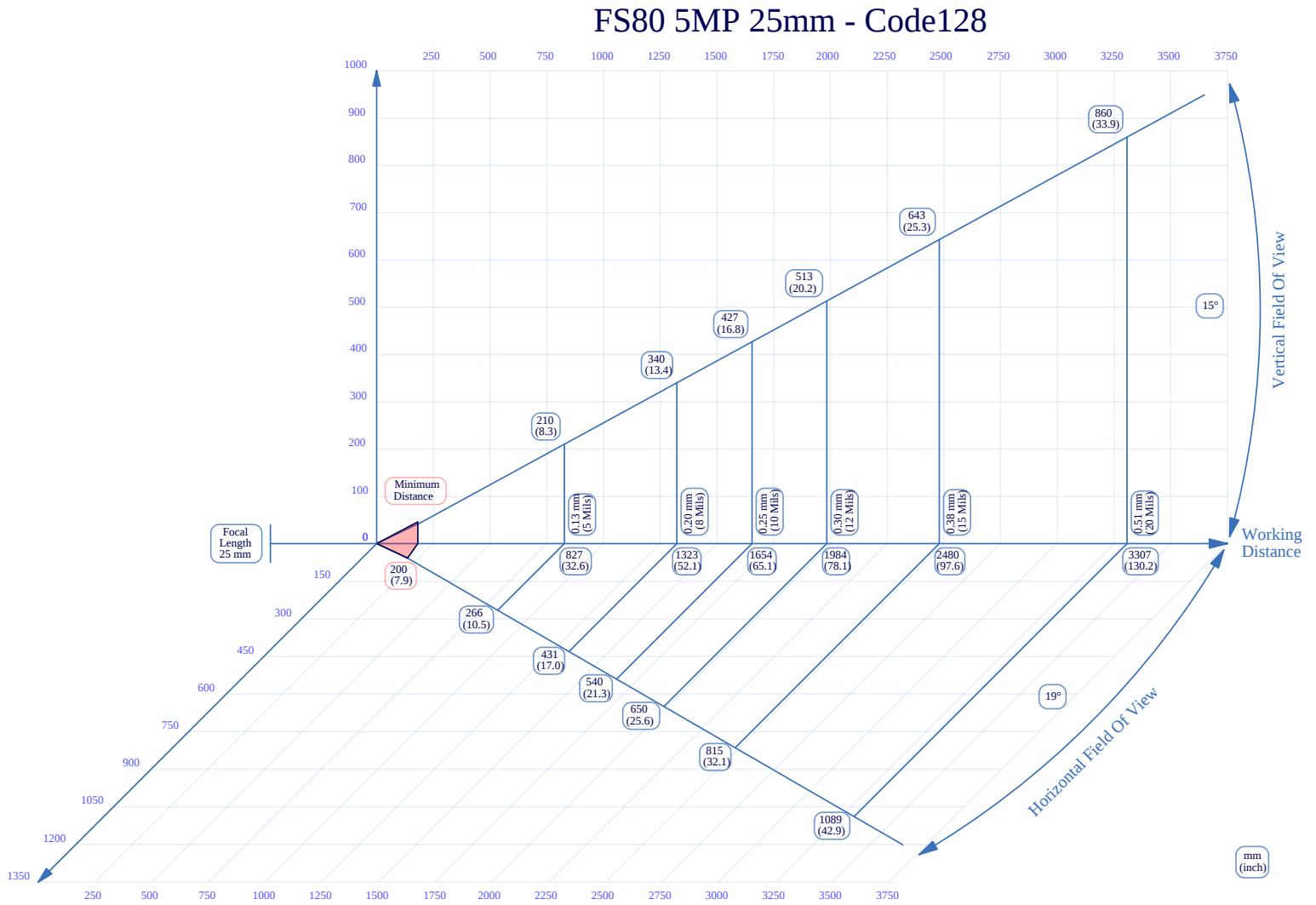
Figure 34 25mm C-Mount Lens Reading Code128
