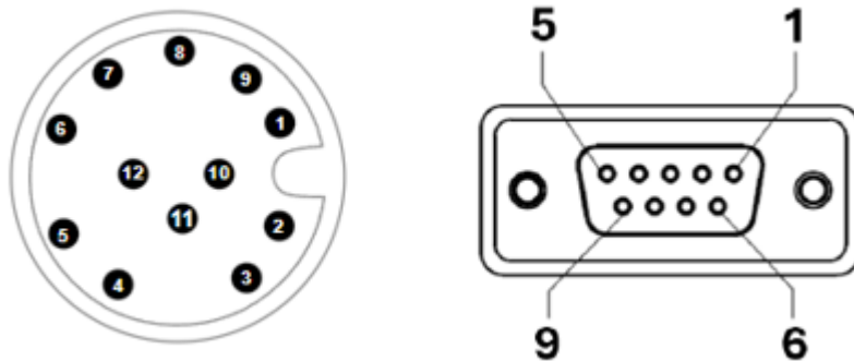
Figure 23 M12 to RS232 DB9 Connector Diagram
