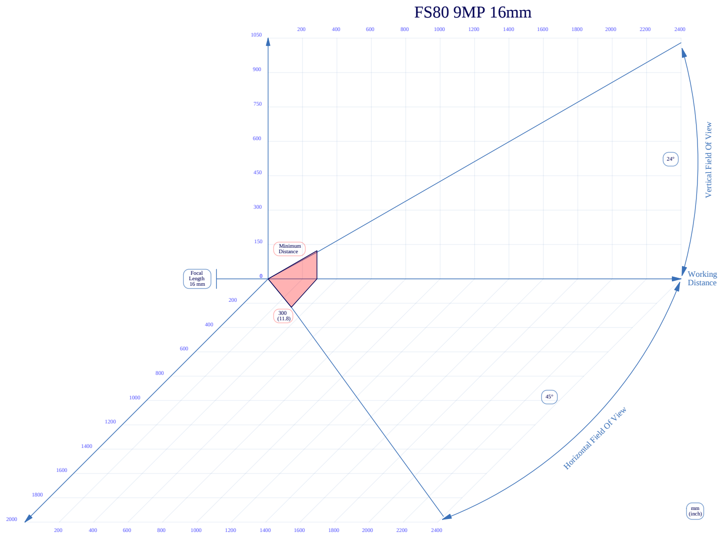
Figure 45 16mm C-Mount Lens Reading Distance
