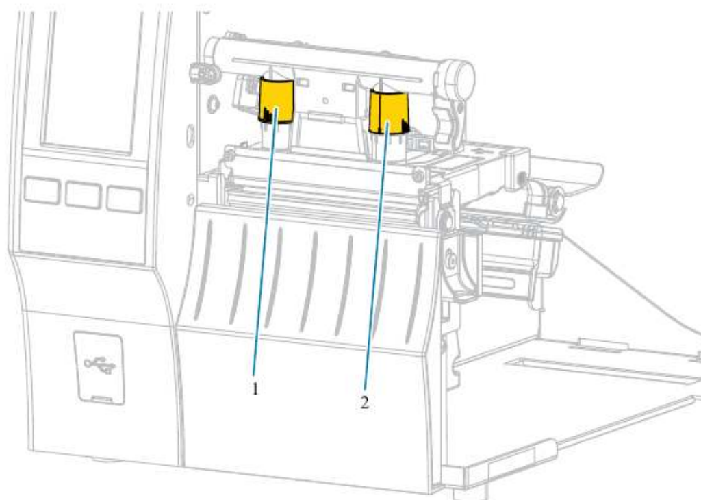
Figure 3 Printhead Pressure Adjustment Dials
